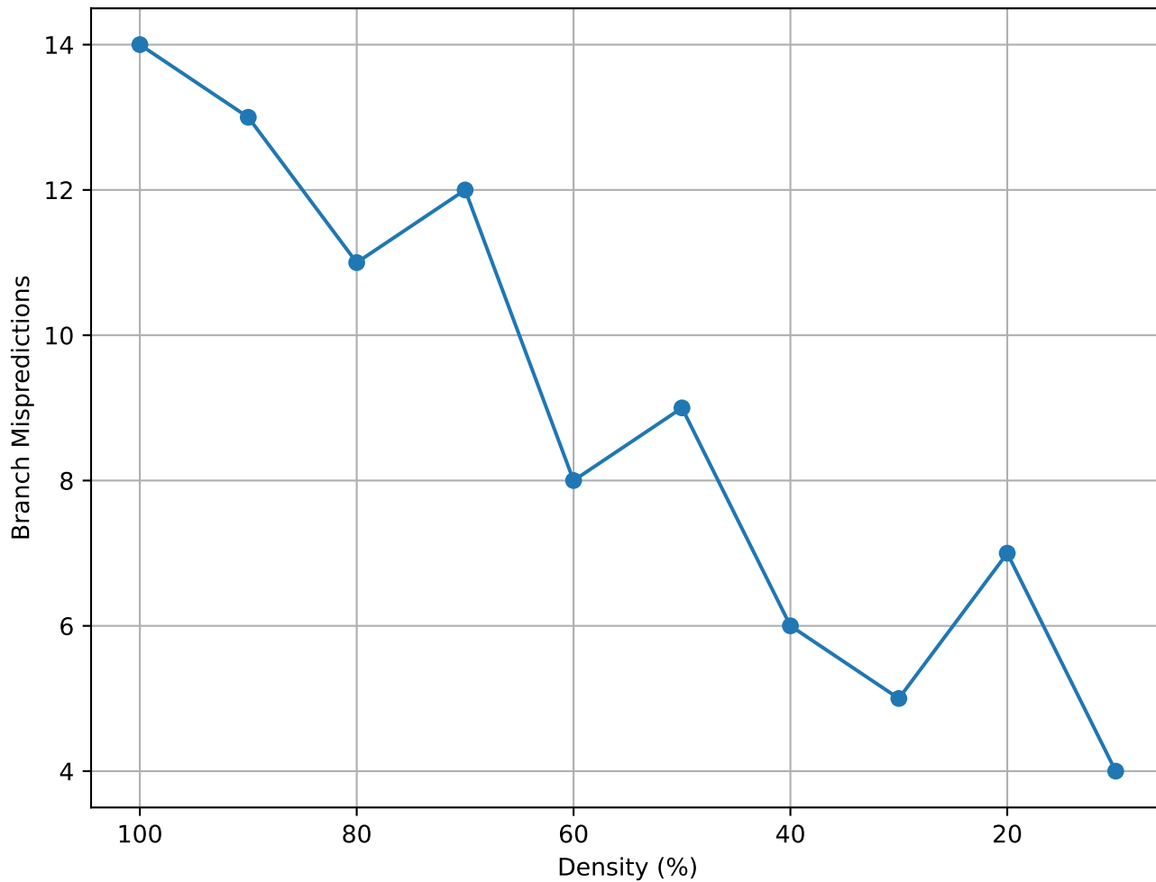
Matrix Density vs Branch Mispredictions (c-32 - consec)
