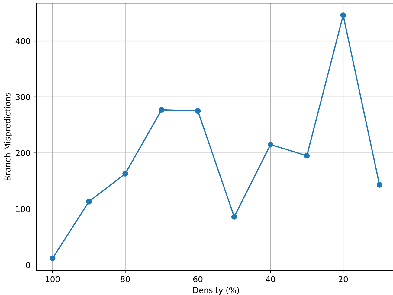
Matrix Density vs Branch Mispredictions (c-32 - random)
