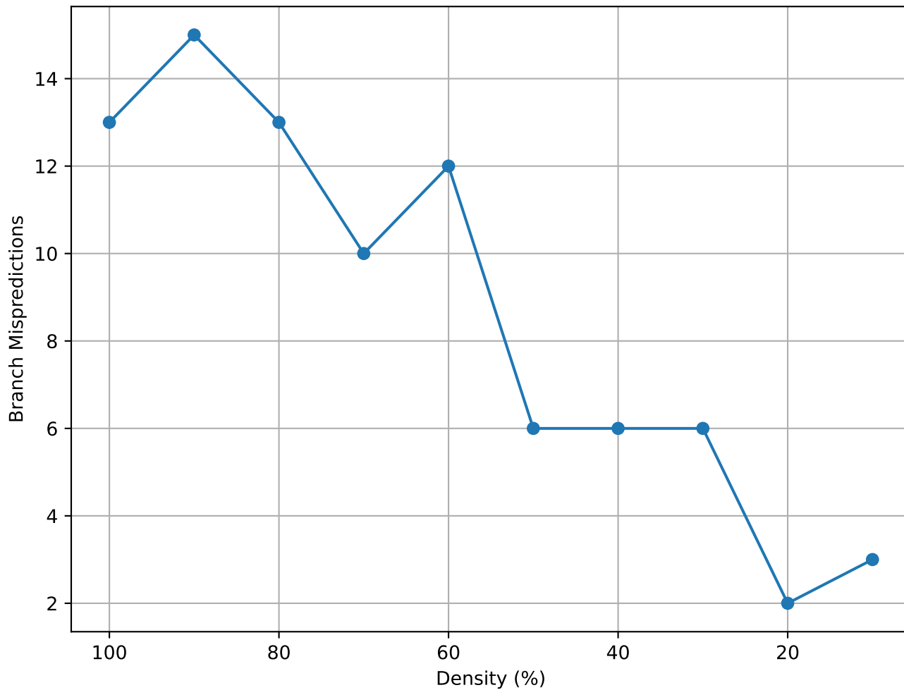
Matrix Density vs Branch Mispredictions (c-32 - truncated)
