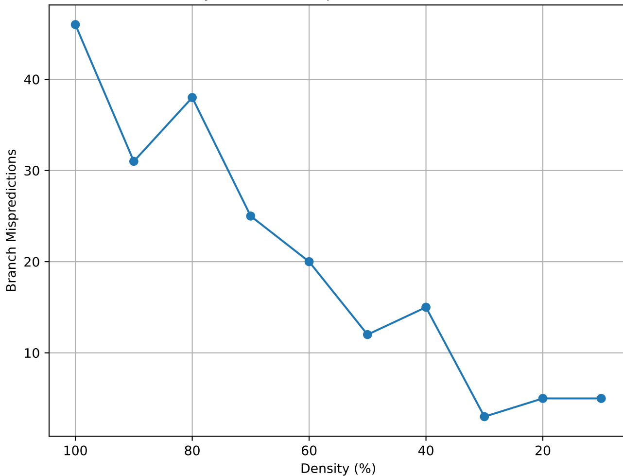
Matrix Density vs Branch Mispredictions (cz2548 - truncated)
