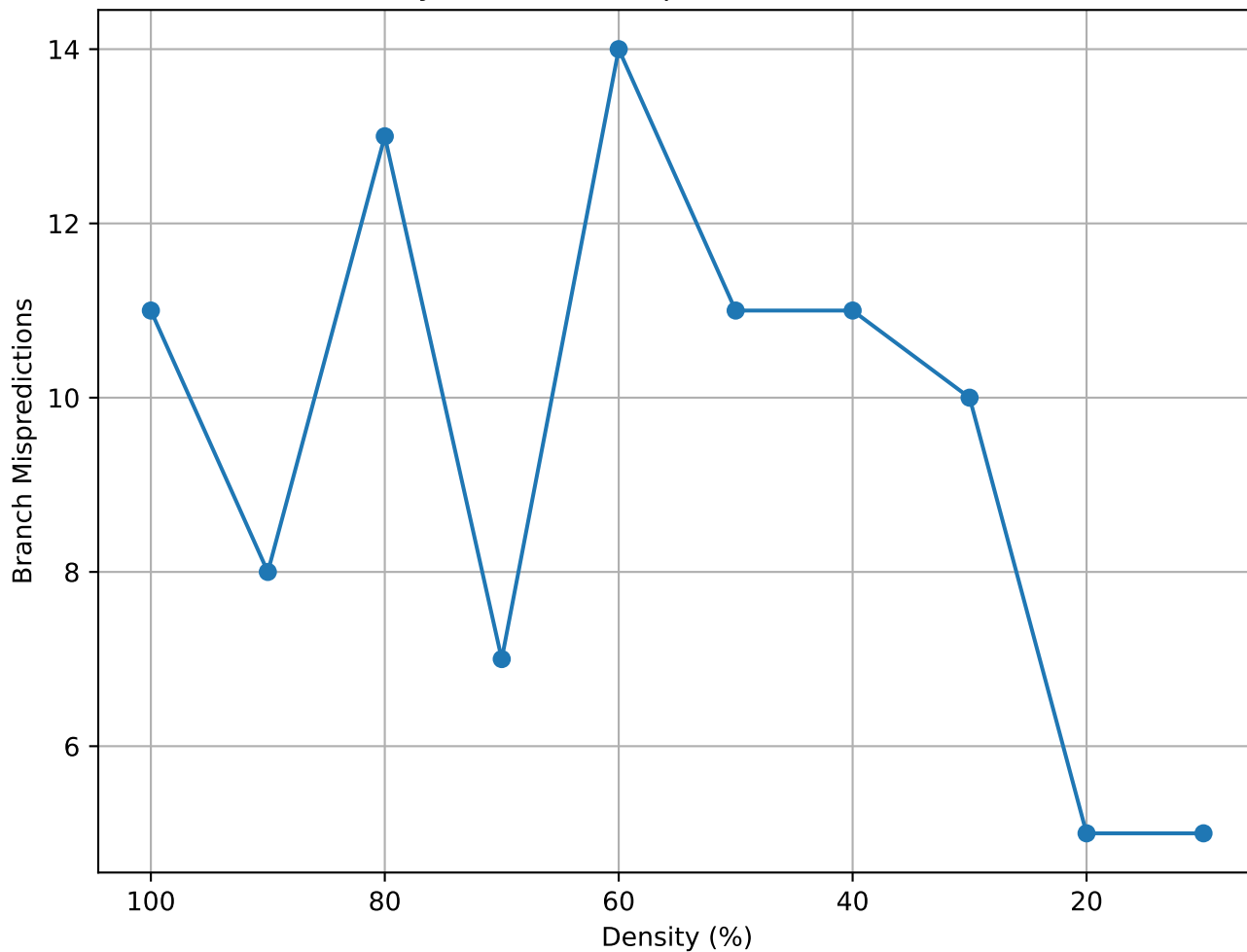
Matrix Density vs Branch Mispredictions (eris1176 - consec)
