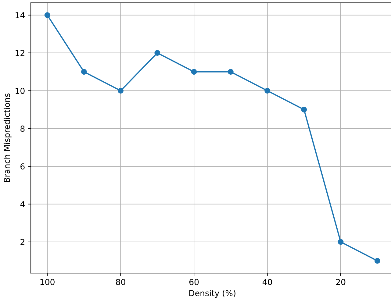
Matrix Density vs Branch Mispredictions (eris1176 - truncated)
