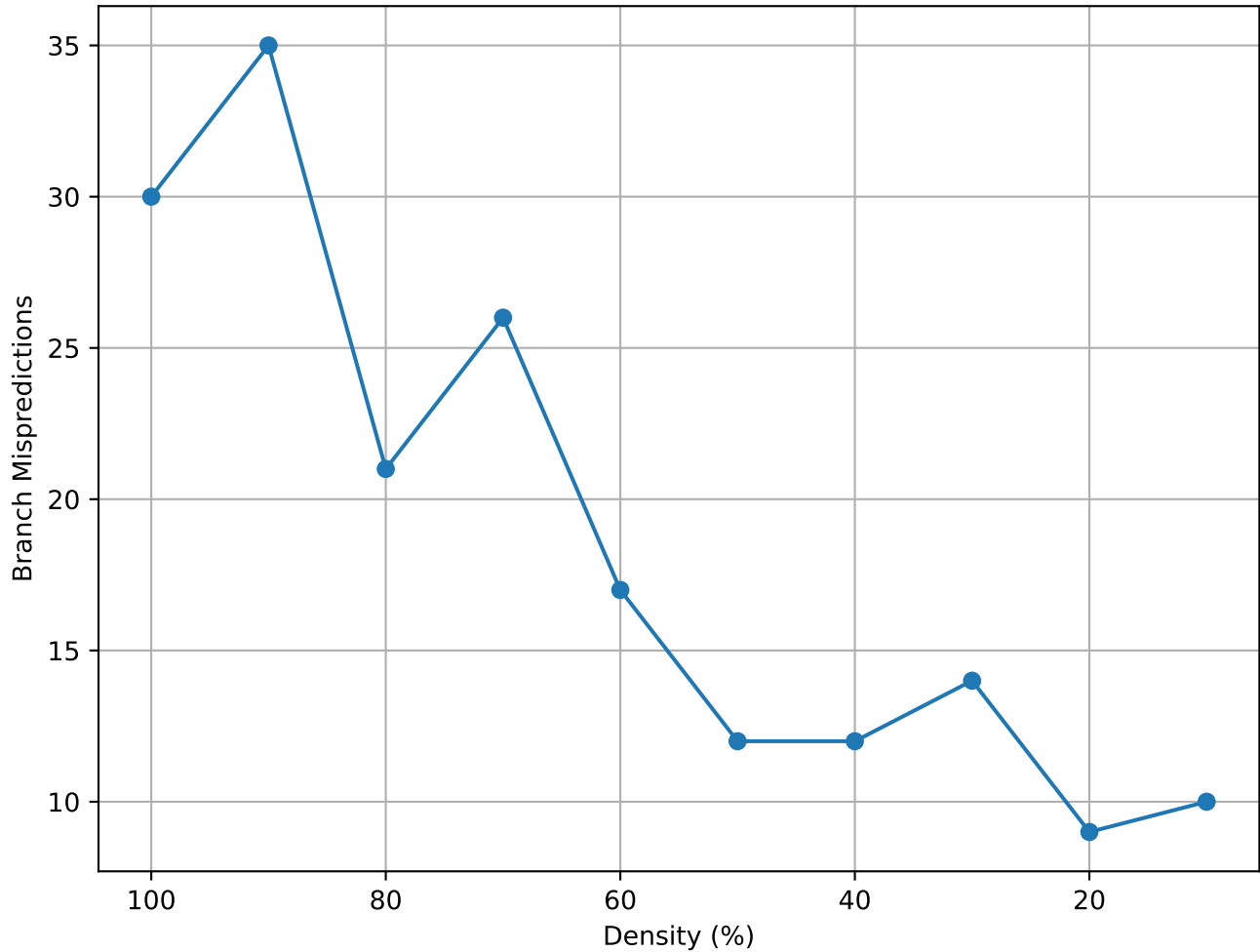
Matrix Density vs Branch Mispredictions (ex10hs - consec)
