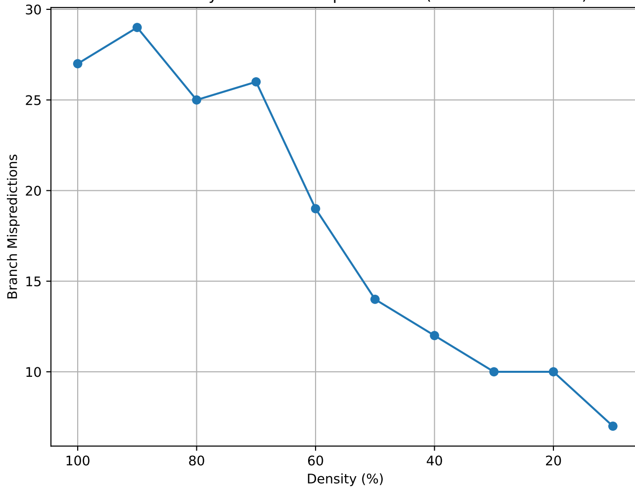
Matrix Density vs Branch Mispredictions (ex10hs - truncated)
