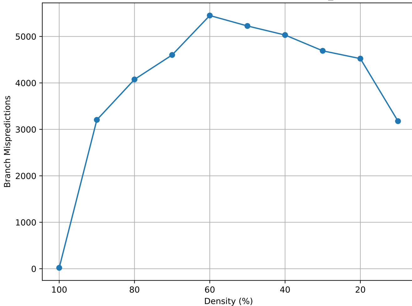
Matrix Density vs Branch Mispredictions (hangGlider_3 - random)
