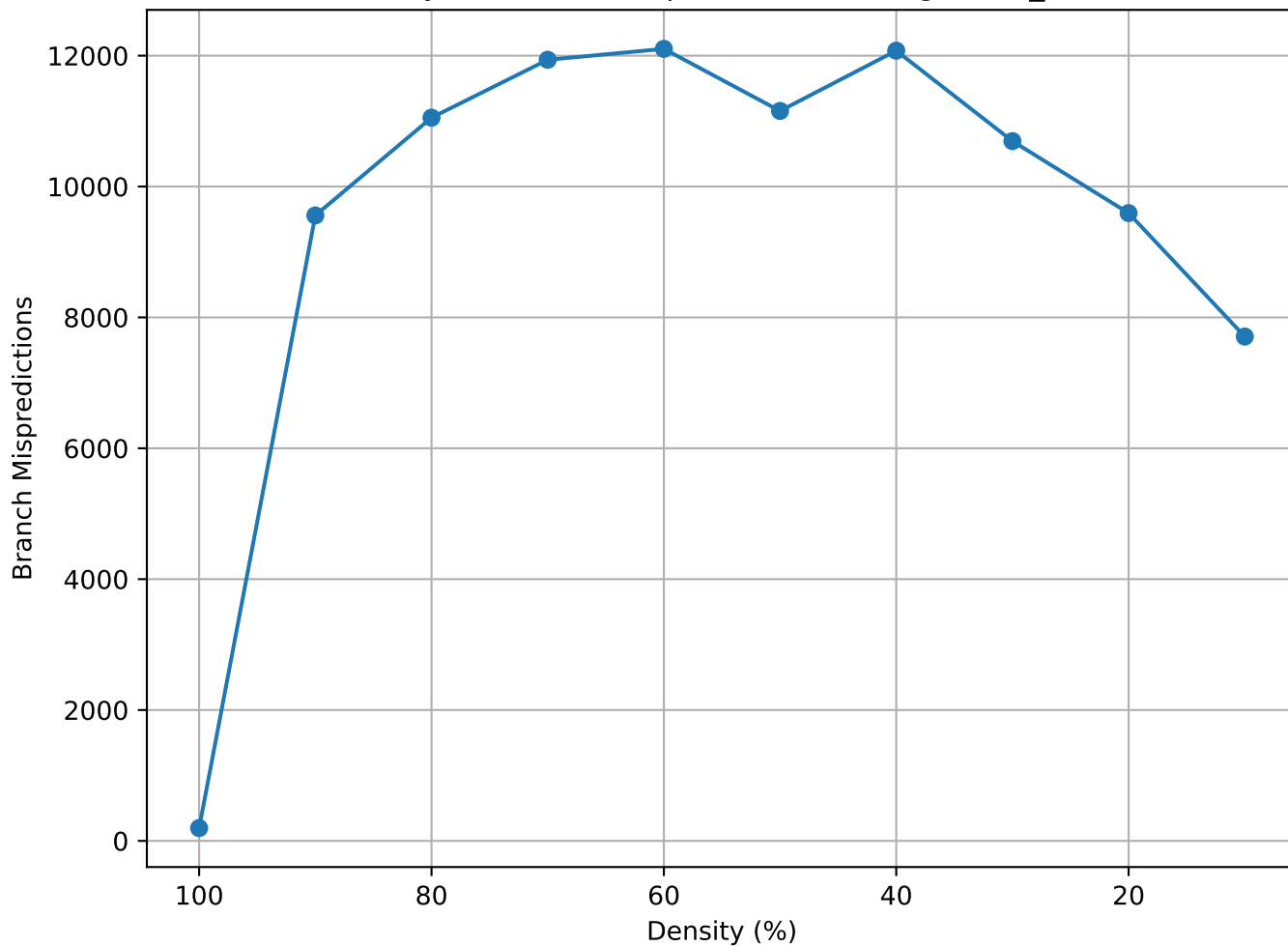
Matrix Density vs Branch Mispredictions (hangGlider_4 - random)
