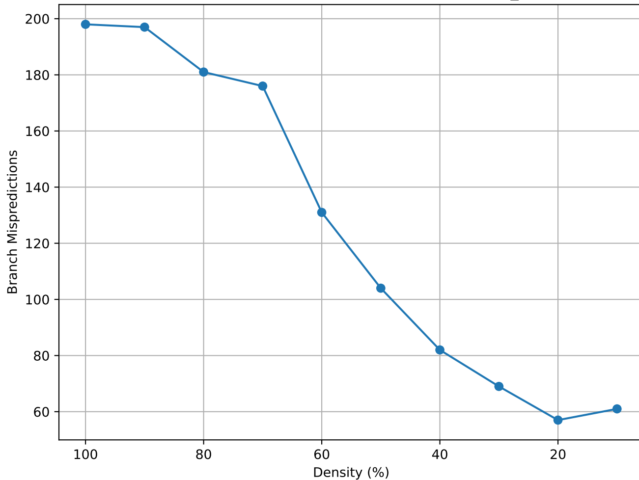
Matrix Density vs Branch Mispredictions (hangGlider_5 - consec)
