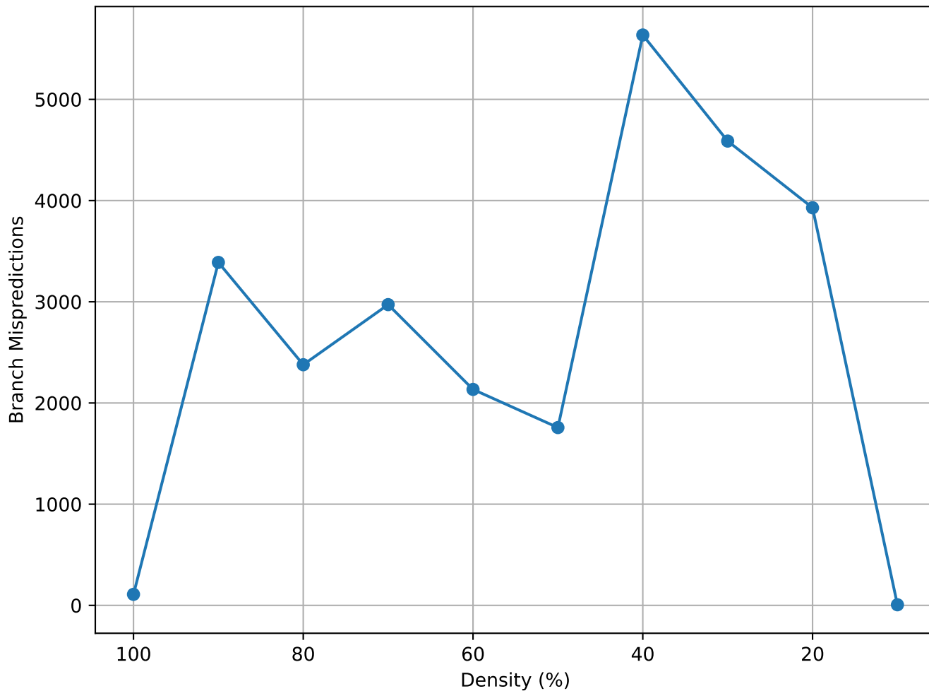
Matrix Density vs Branch Mispredictions (heart1 - random)
