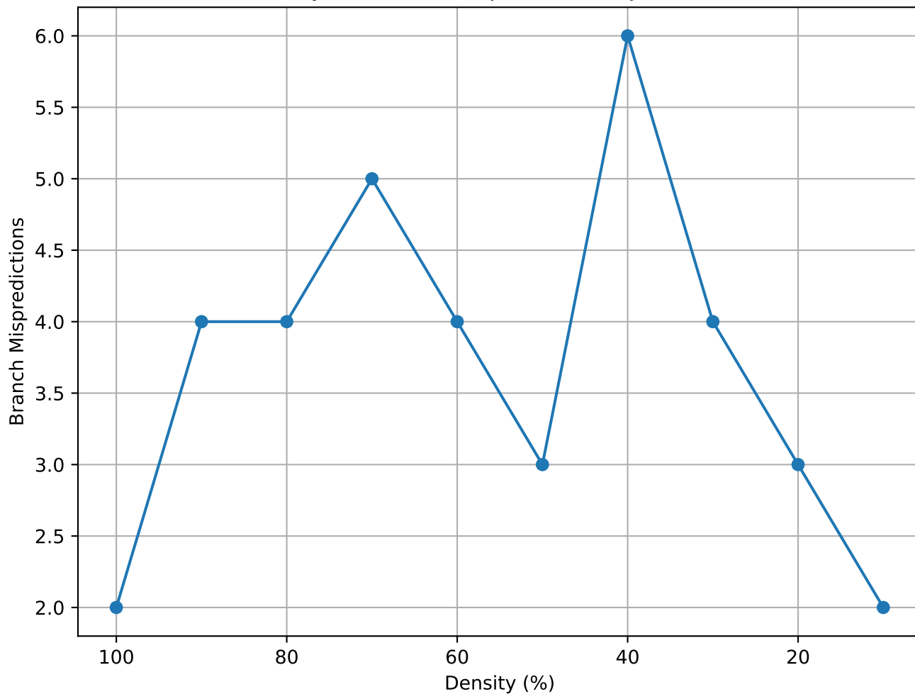
Matrix Density vs Branch Mispredictions (jendrec1 - consec)
