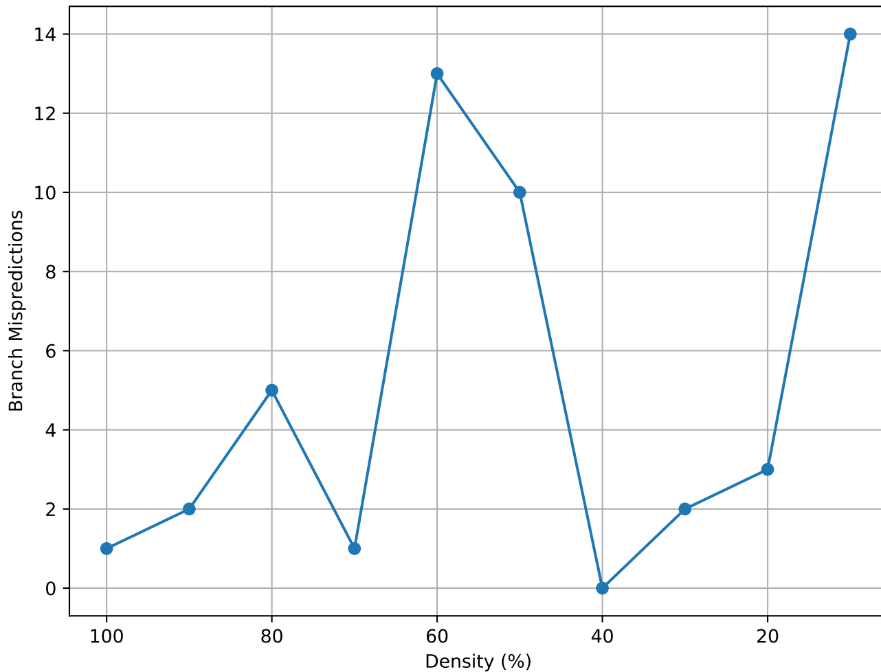
Matrix Density vs Branch Mispredictions (jendrec1 - random)
