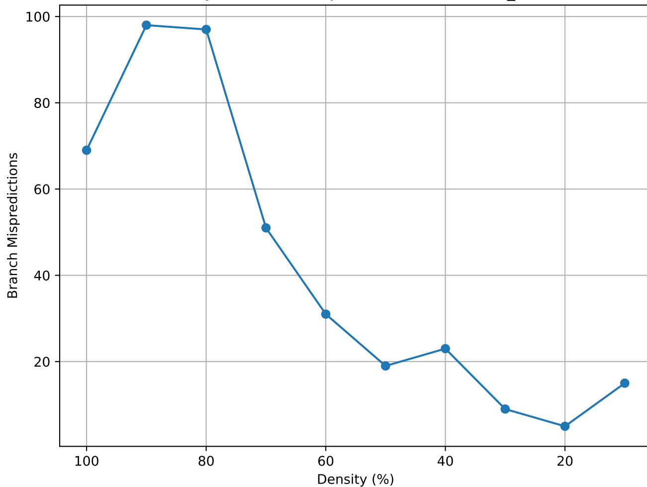
Matrix Density vs Branch Mispredictions (lowThrust_10 - consec)
