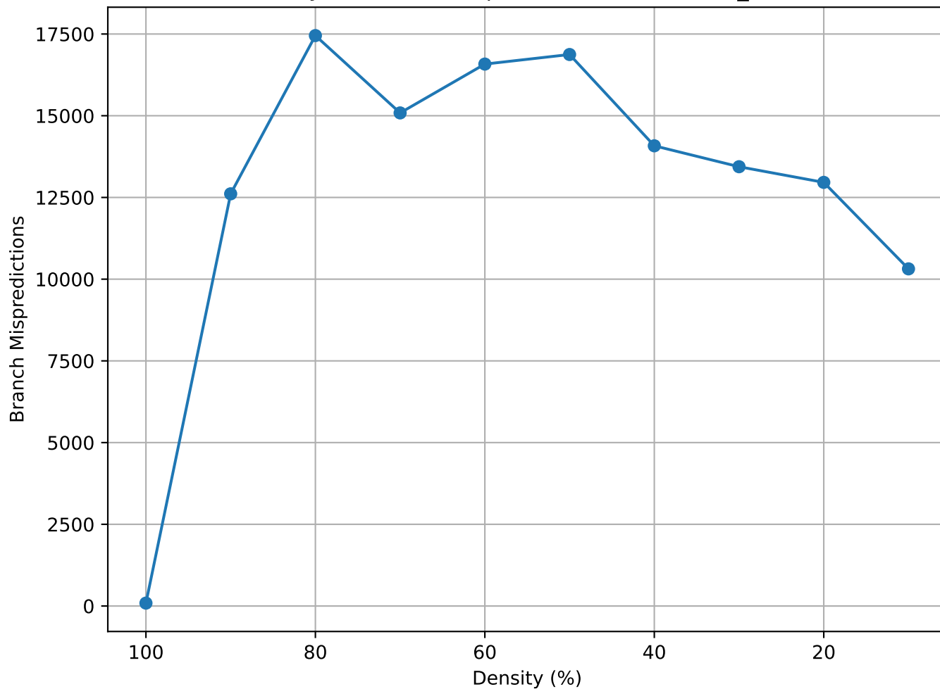
Matrix Density vs Branch Mispredictions (lowThrust_10 - random)
