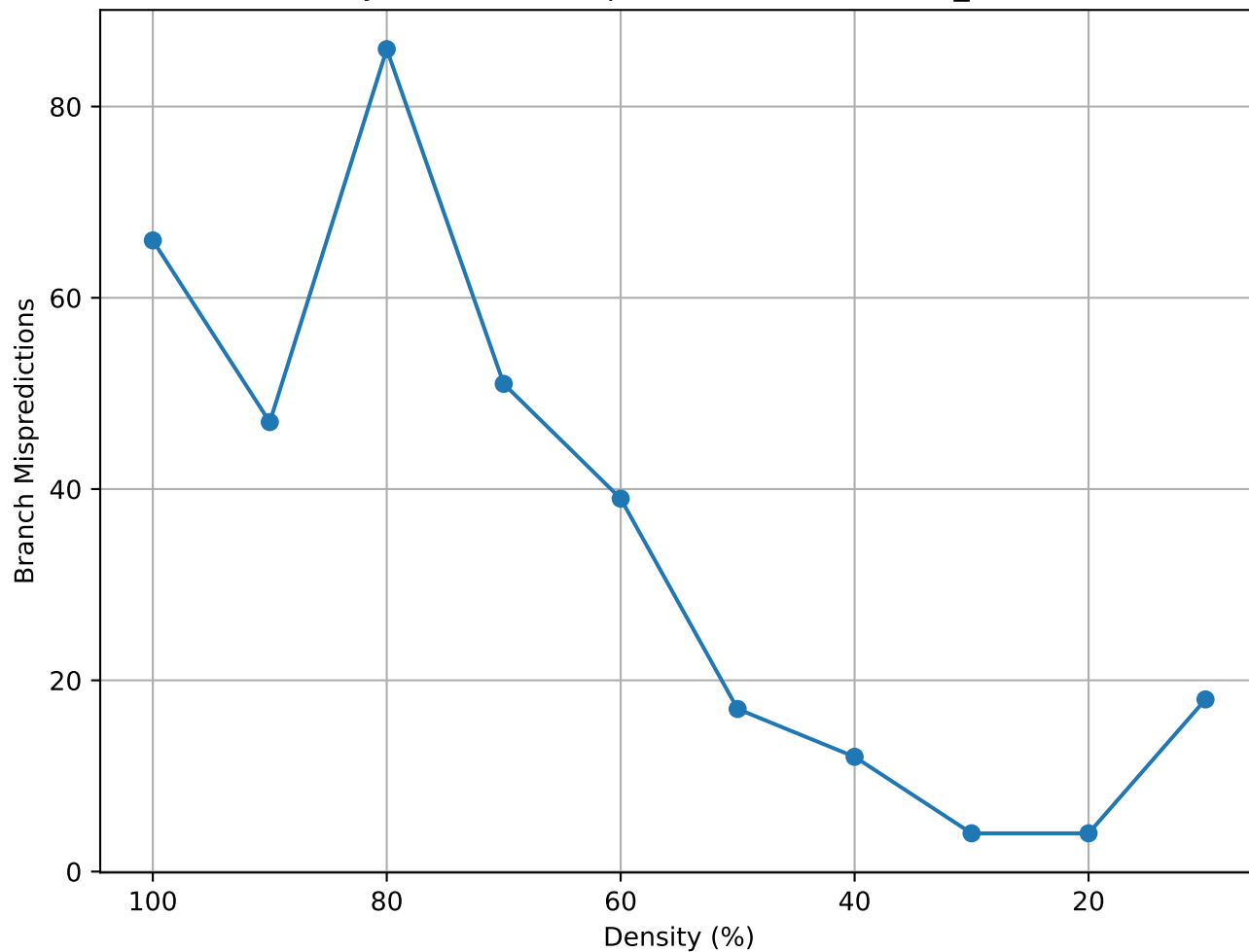
Matrix Density vs Branch Mispredictions (lowThrust_10 - truncated)
