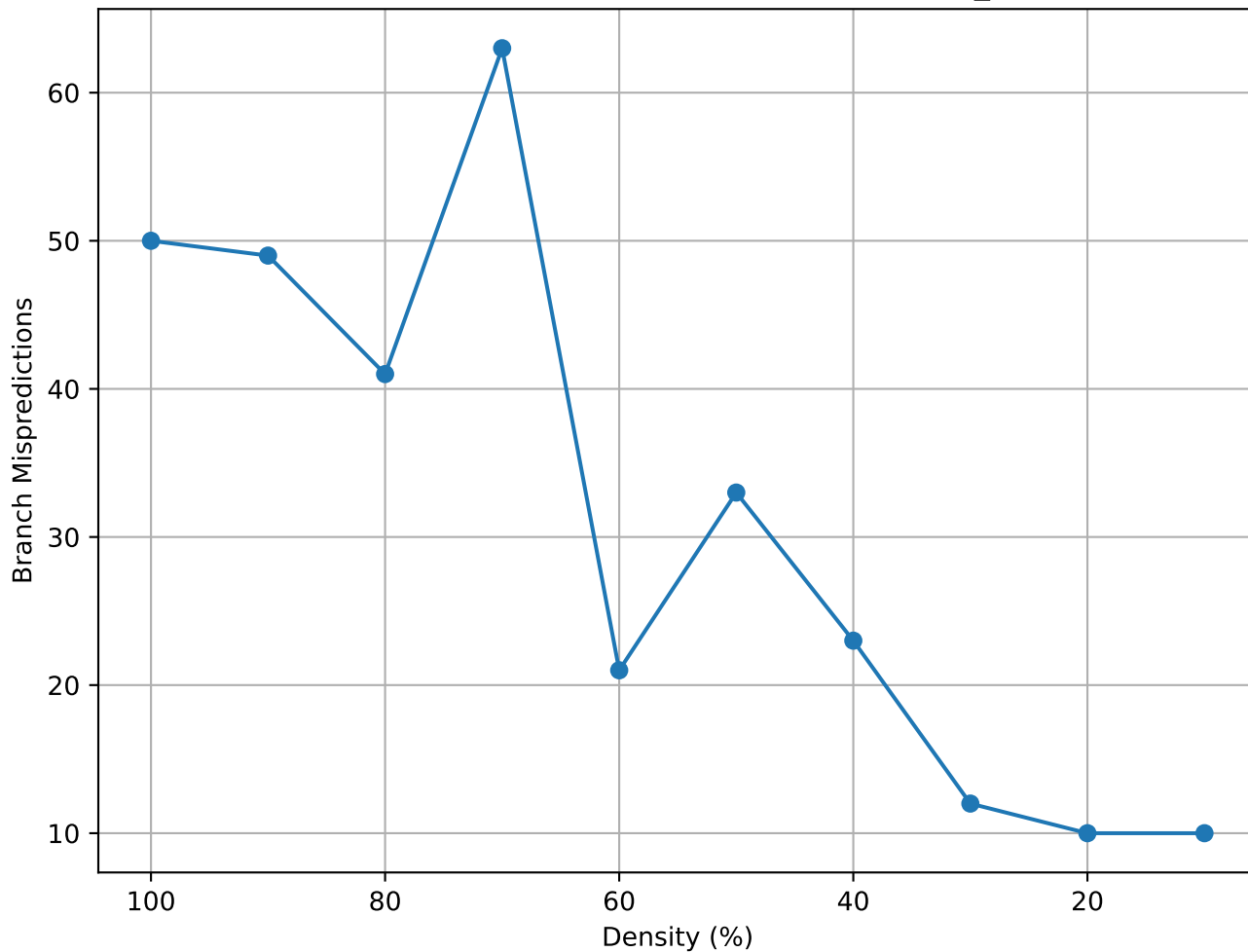
Matrix Density vs Branch Mispredictions (lowThrust_11 - consec)
