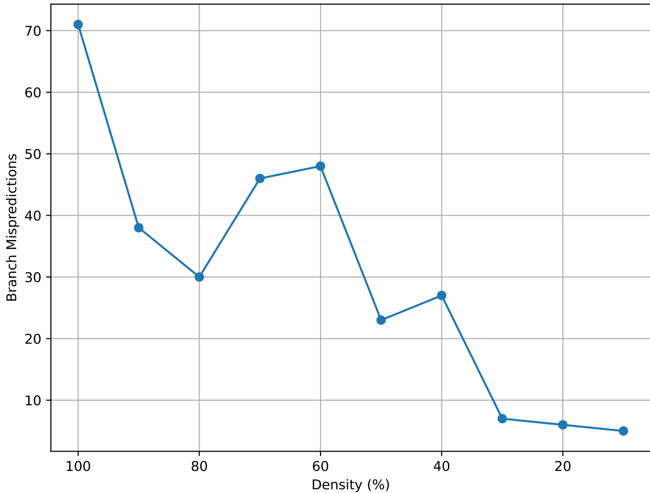
Matrix Density vs Branch Mispredictions (lowThrust_12 - consec)
