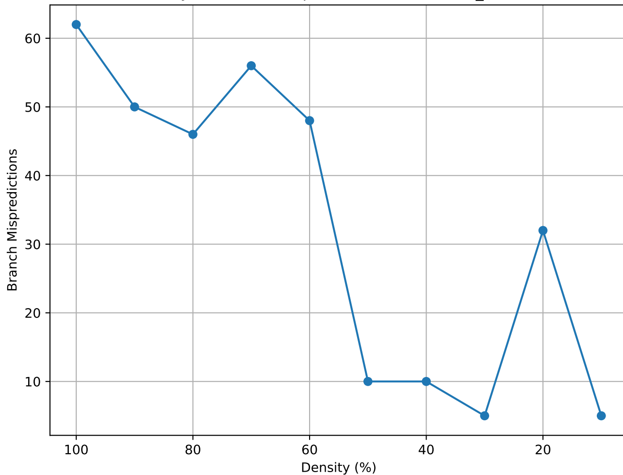
Matrix Density vs Branch Mispredictions (lowThrust_12 - truncated)
