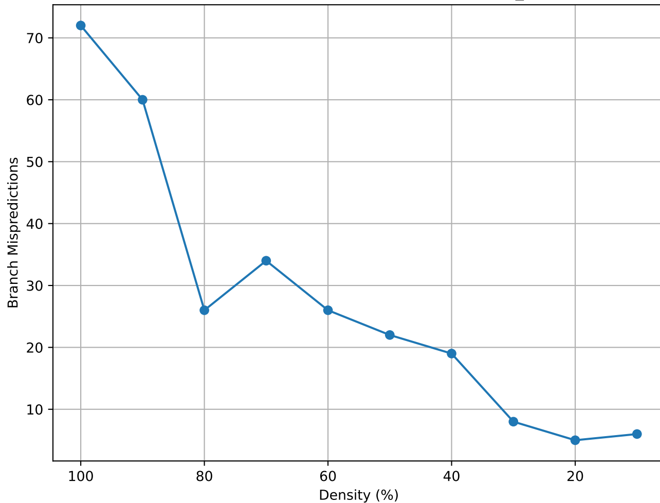
Matrix Density vs Branch Mispredictions (lowThrust_13 - consec)
