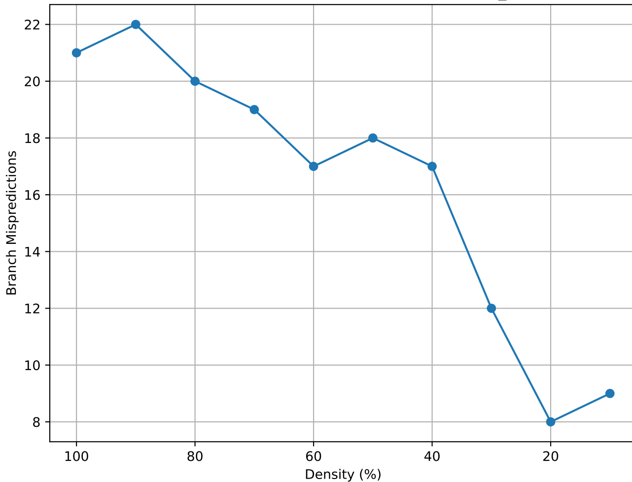
Matrix Density vs Branch Mispredictions (lowThrust_3 - consec)
