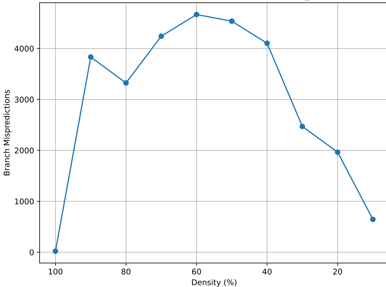
Matrix Density vs Branch Mispredictions (lowThrust_3 - random)
