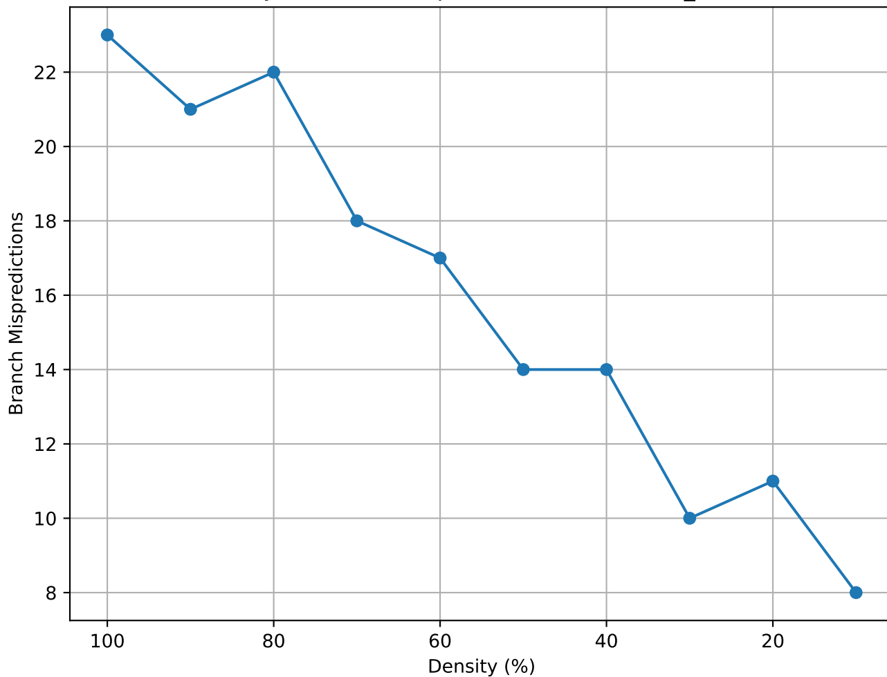
Matrix Density vs Branch Mispredictions (lowThrust_3 - truncated)
