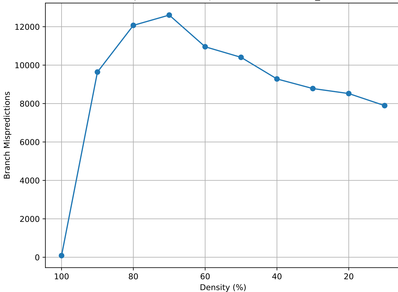
Matrix Density vs Branch Mispredictions (lowThrust_4 - random)
