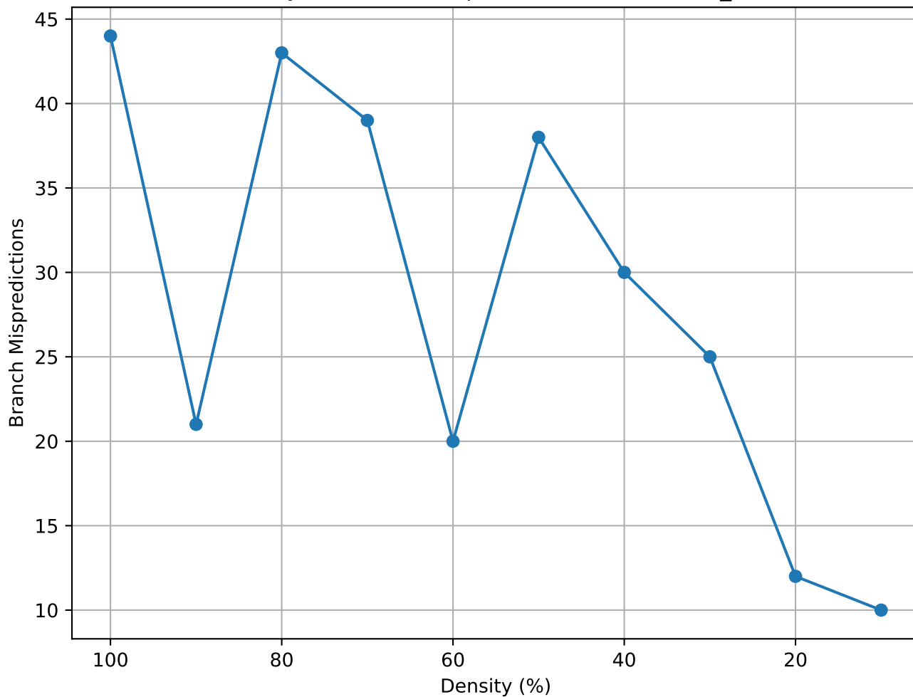
Matrix Density vs Branch Mispredictions (lowThrust_5 - consec)
