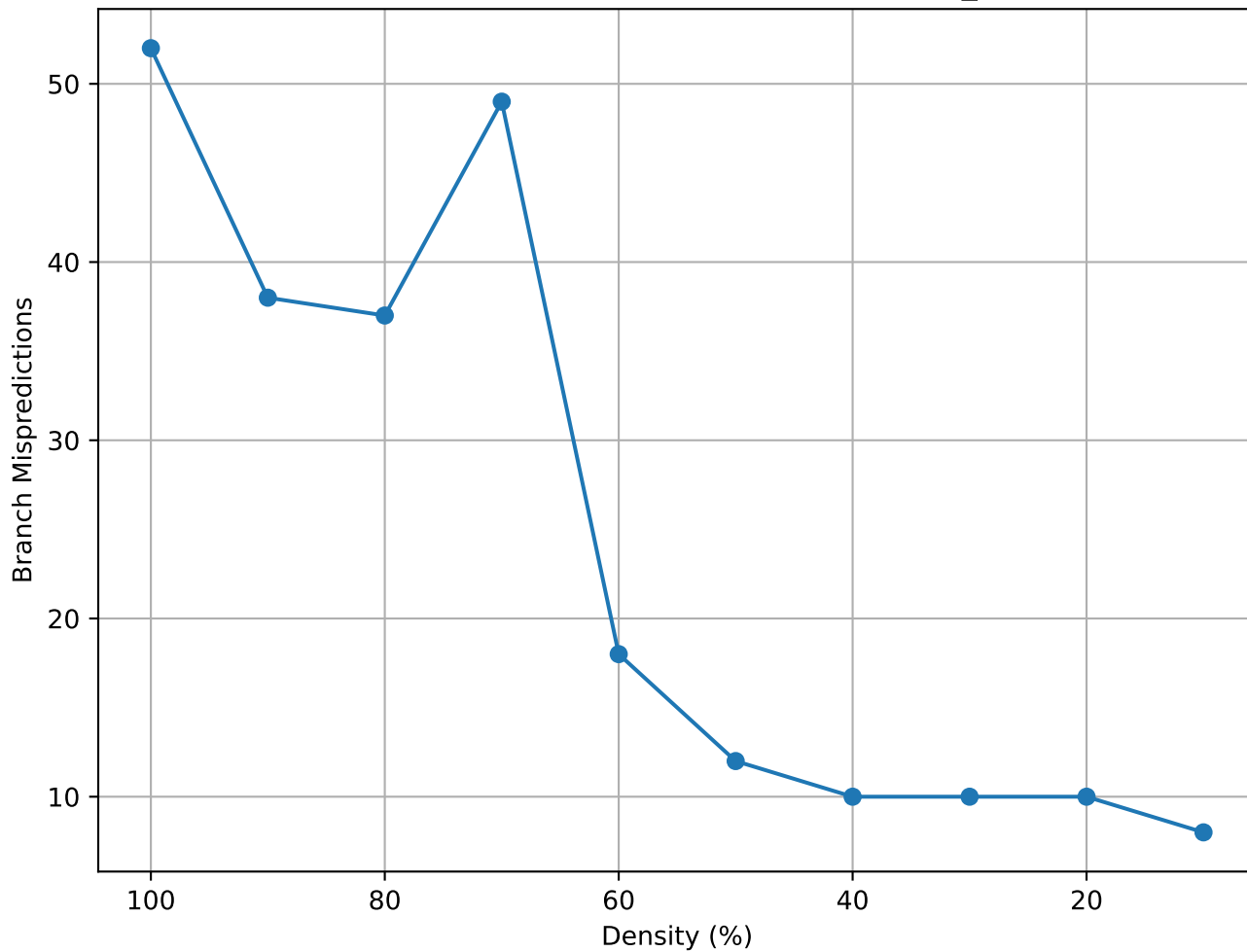
Matrix Density vs Branch Mispredictions (lowThrust_5 - truncated)
