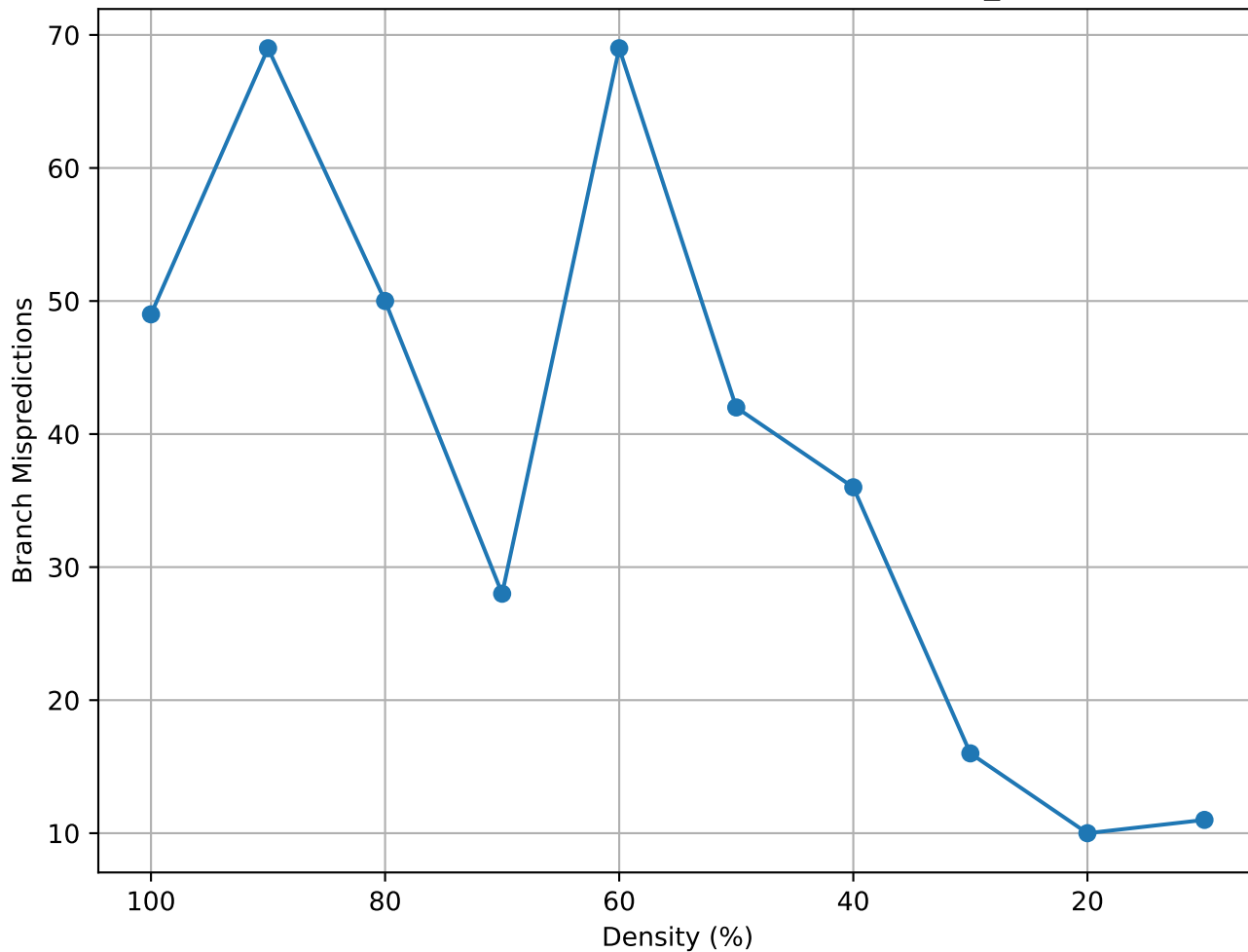
Matrix Density vs Branch Mispredictions (lowThrust_6 - consec)
