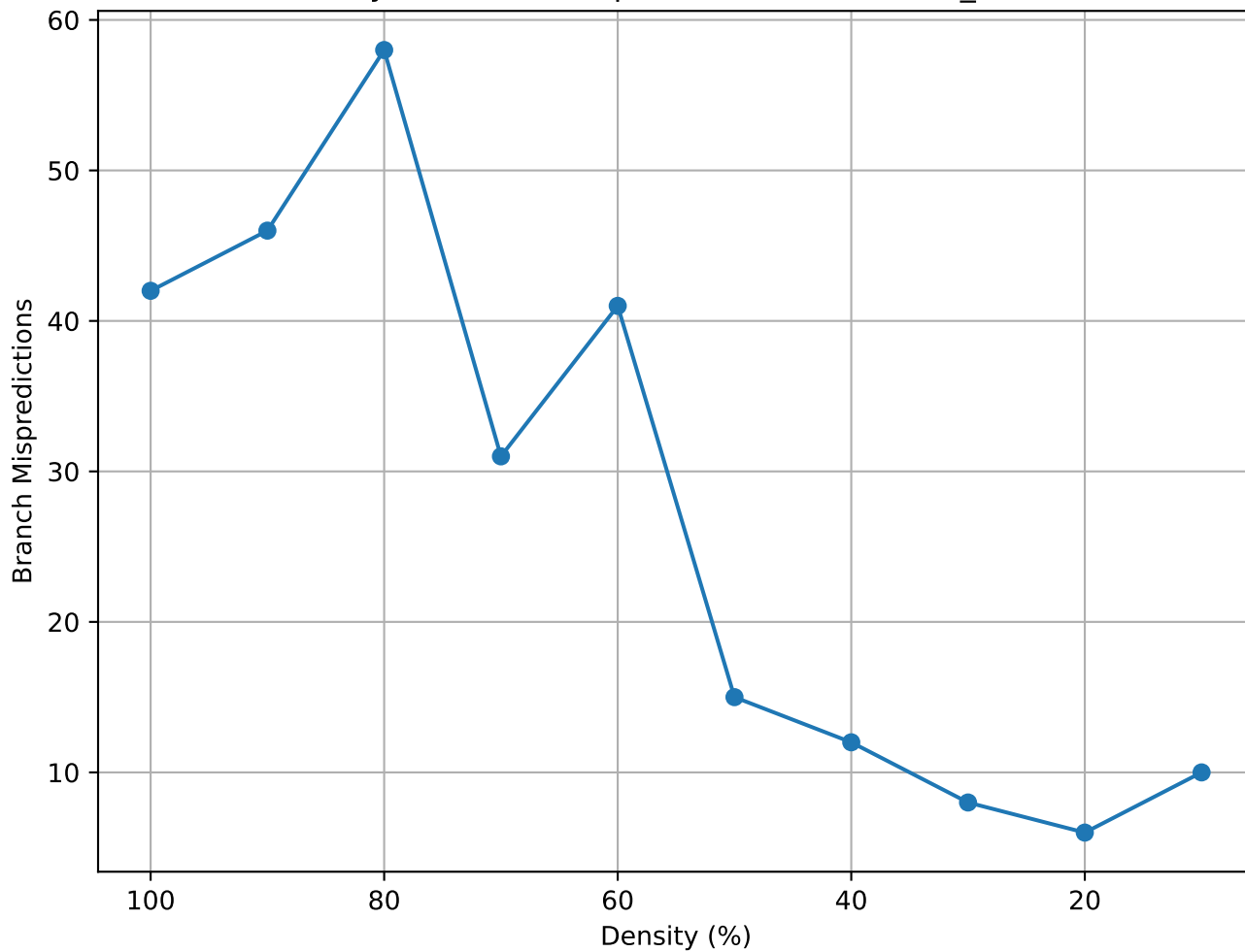
Matrix Density vs Branch Mispredictions (lowThrust_7 - truncated)
