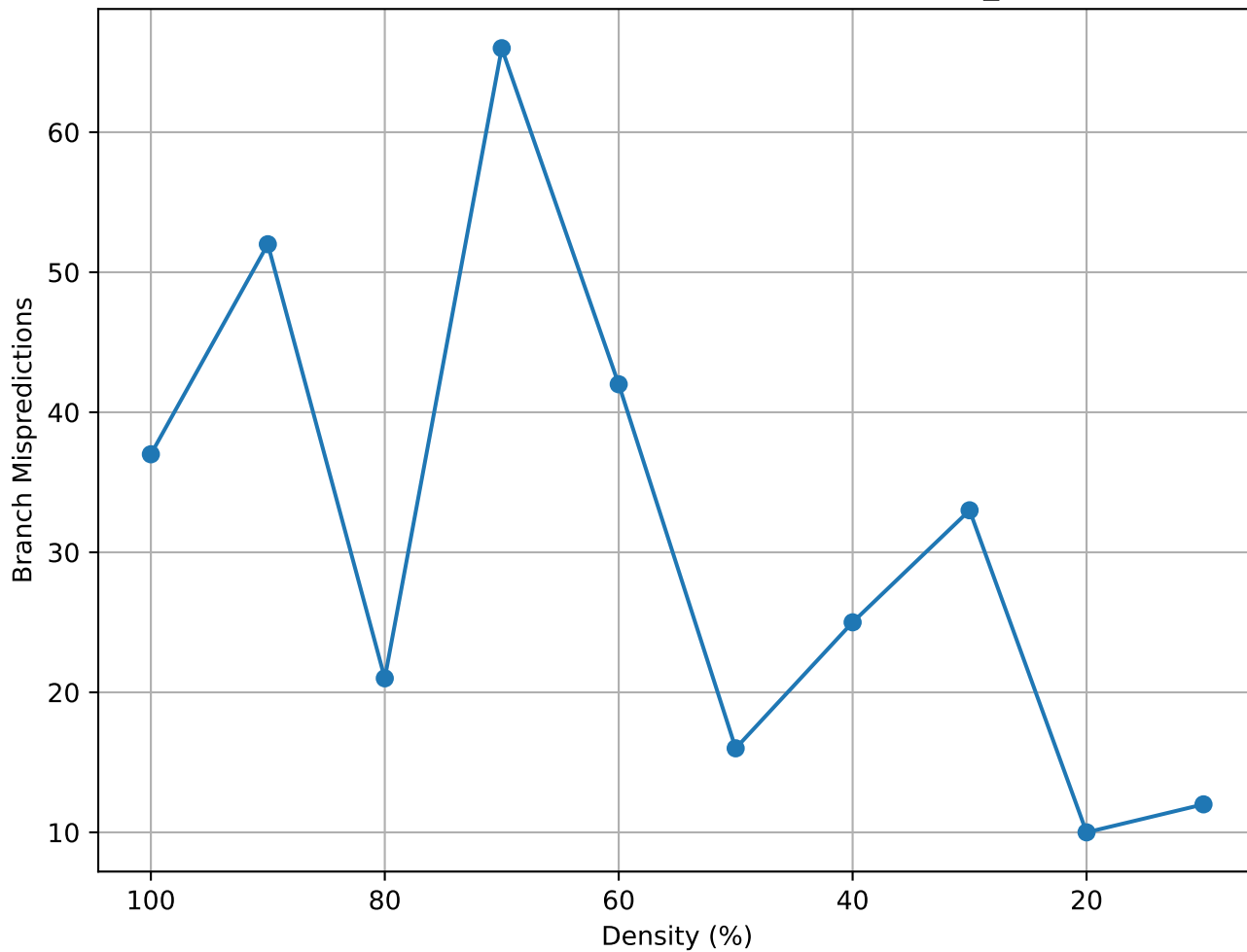
Matrix Density vs Branch Mispredictions (lowThrust_8 - consec)
