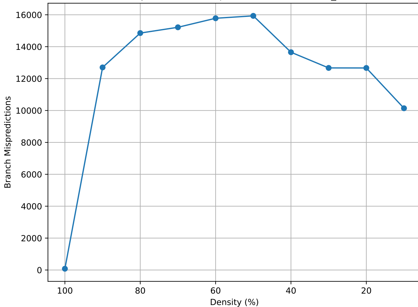
Matrix Density vs Branch Mispredictions (lowThrust_8 - random)
