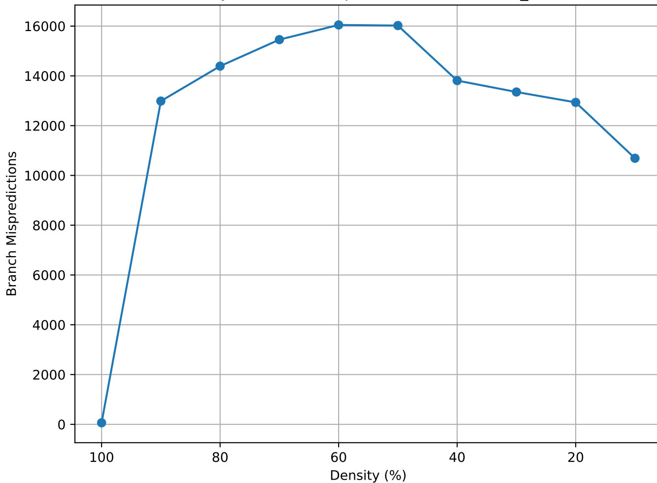
Matrix Density vs Branch Mispredictions (lowThrust_9 - random)
