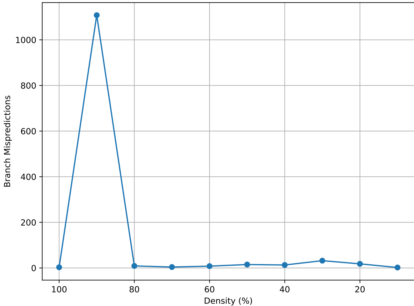
Matrix Density vs Branch Mispredictions (lp_fit2p - random)
