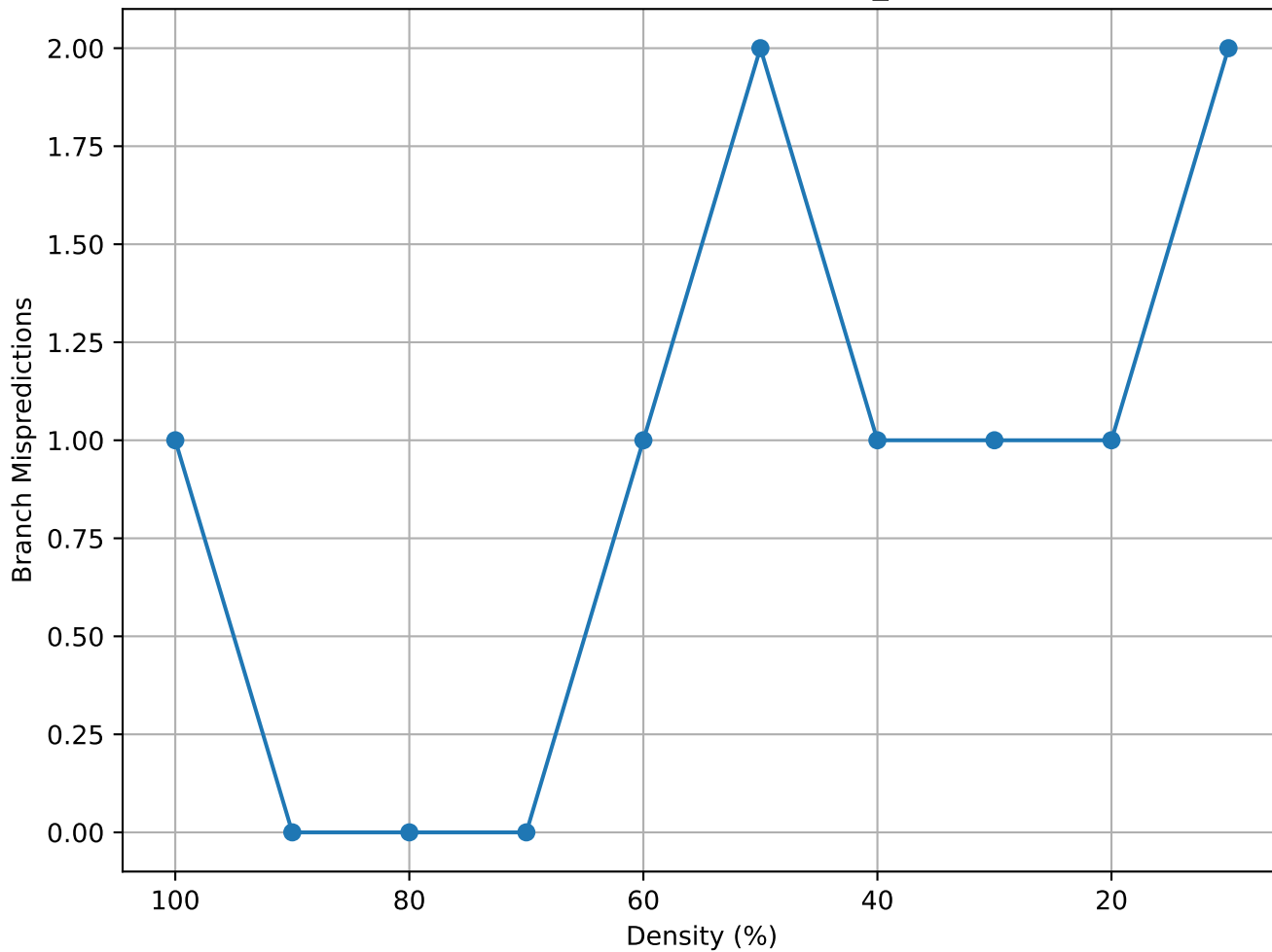
Matrix Density vs Branch Mispredictions (lp_wood1p - truncated)
