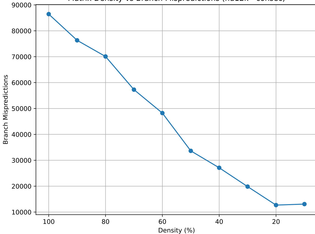
Matrix Density vs Branch Mispredictions (nd12k - consec)
