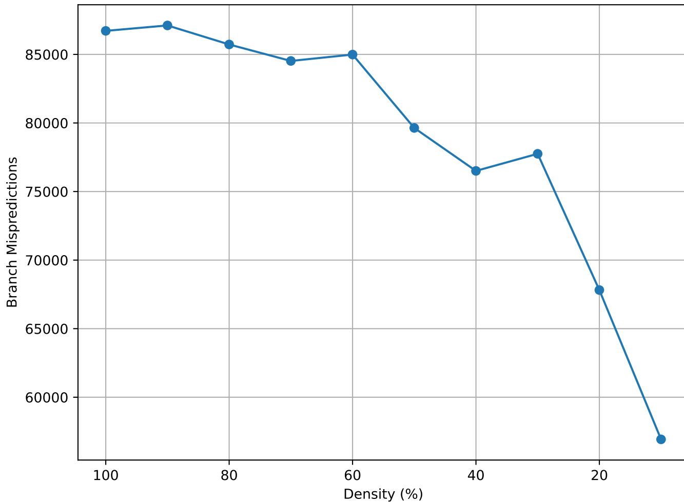
Matrix Density vs Branch Mispredictions (nd12k - random)
