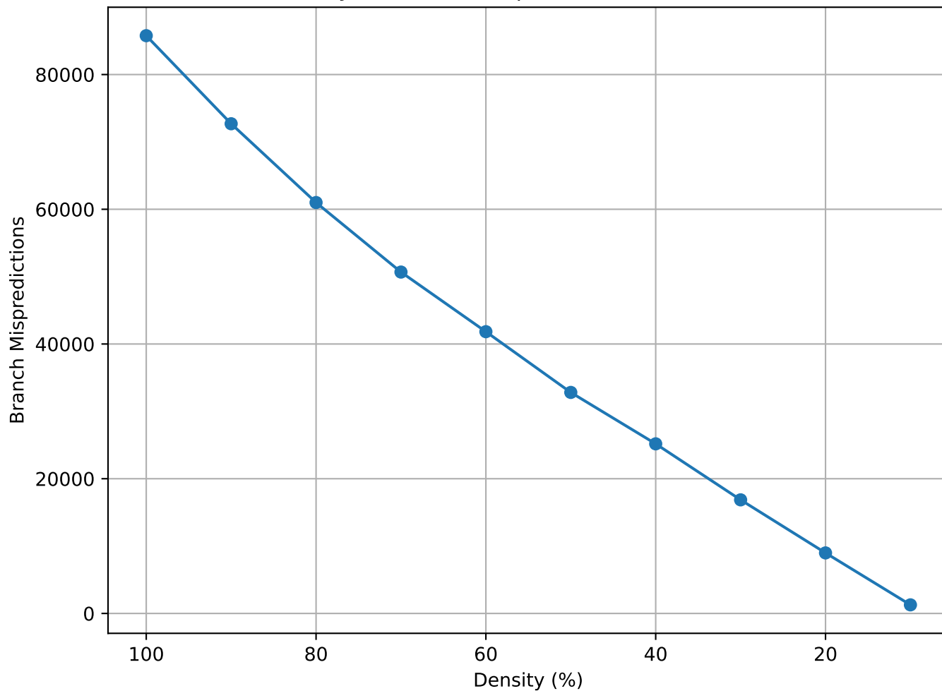
Matrix Density vs Branch Mispredictions (nd12k - truncated)
