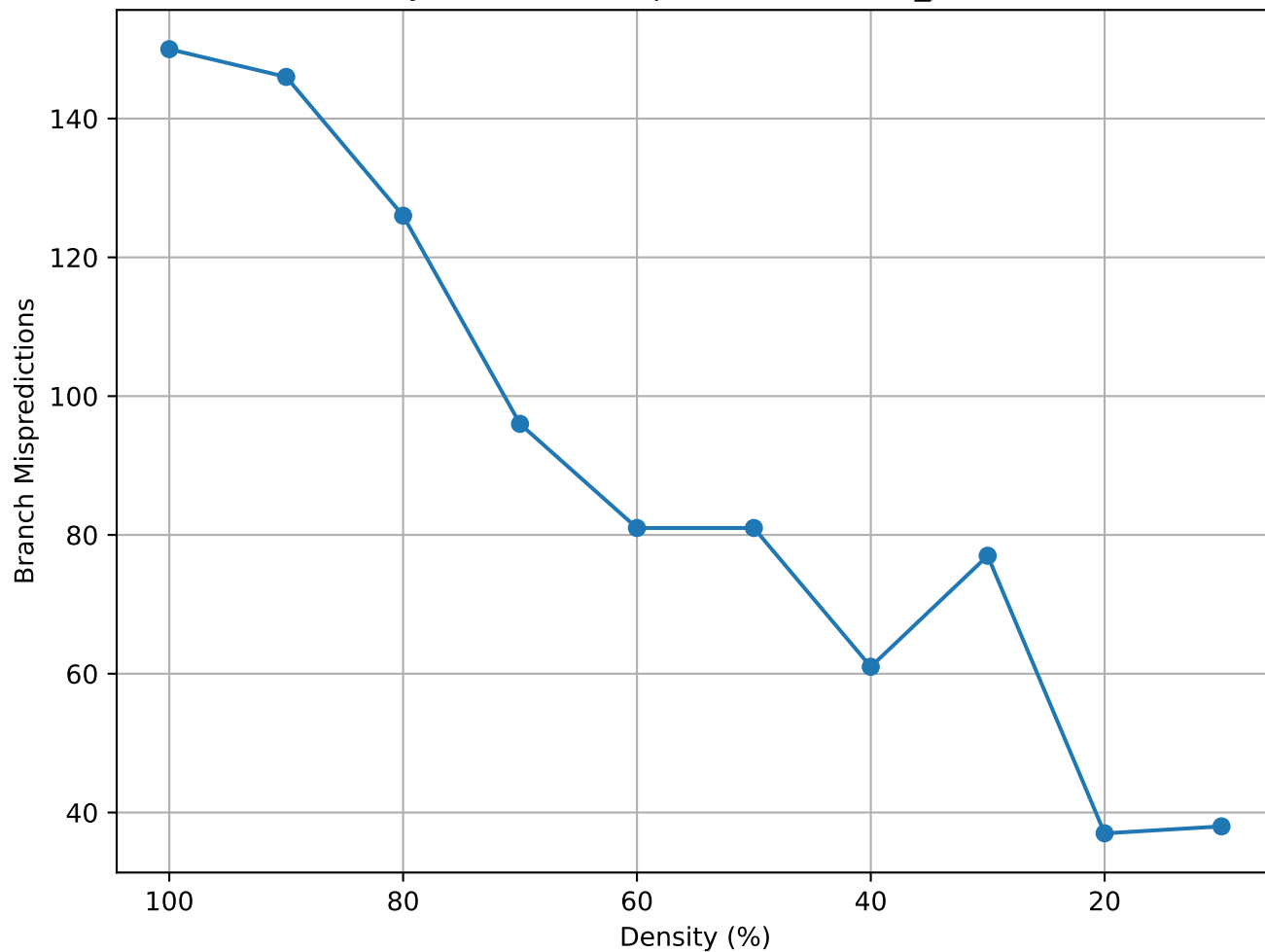
Matrix Density vs Branch Mispredictions (std1_Jac2 - truncated)
