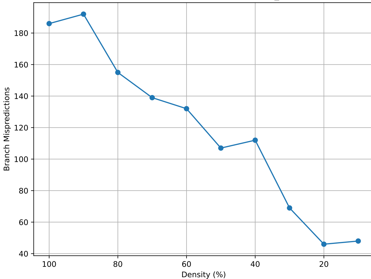
Matrix Density vs Branch Mispredictions (std1_Jac3 - consec)
