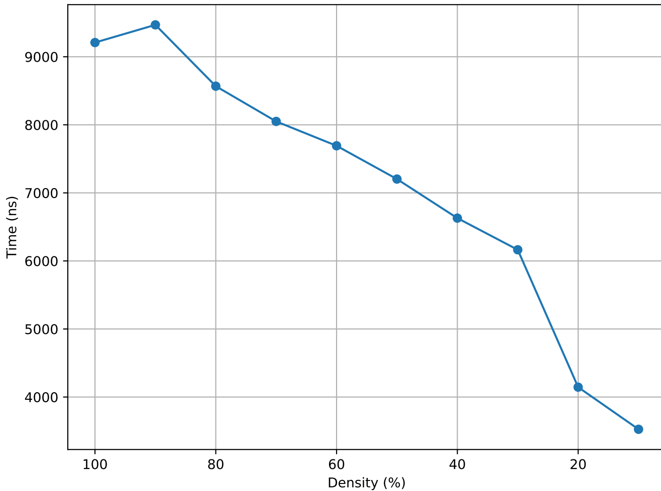
Matrix Density vs Time (Sieber - random)
