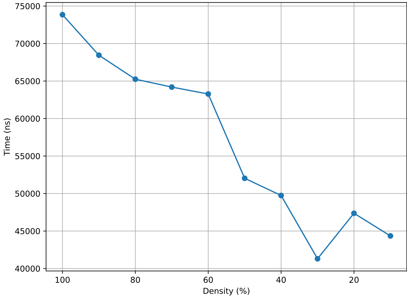
Matrix Density vs Time (bloweybl - consec)
