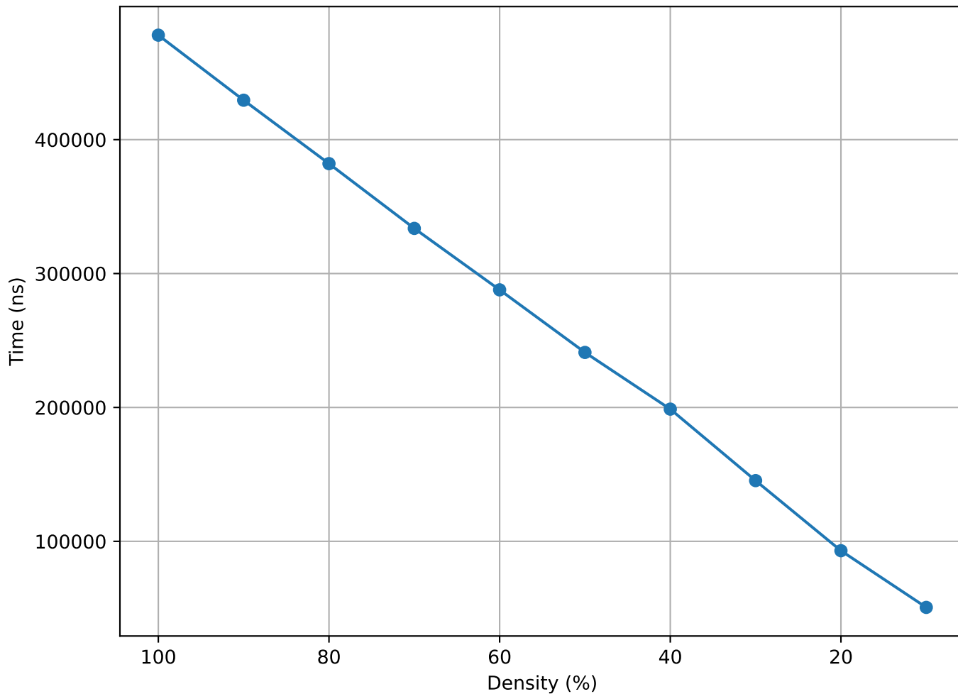
Matrix Density vs Time (heart1 - truncated)
