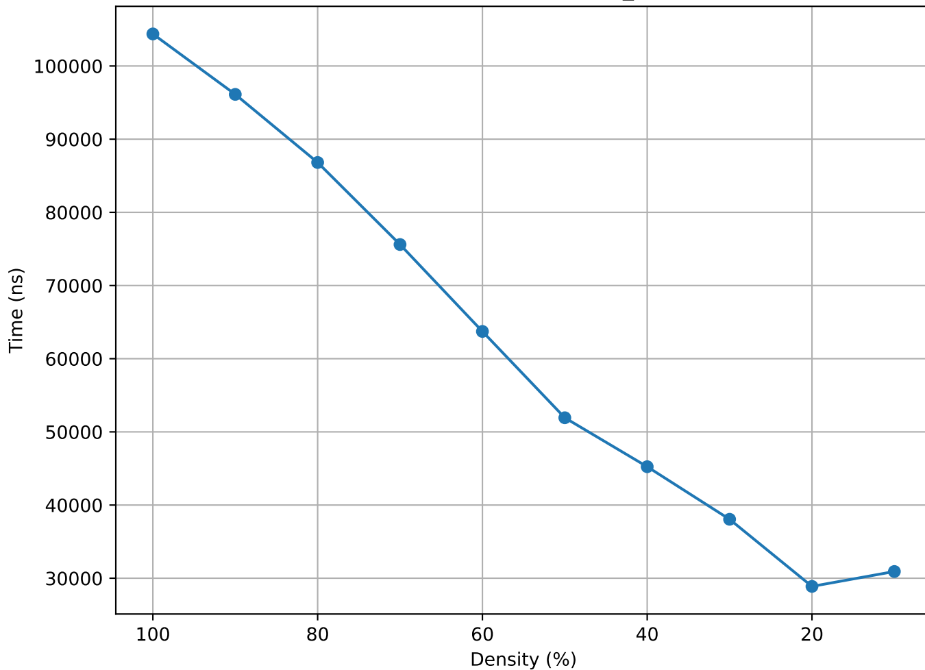
Matrix Density vs Time (lowThrust_11 - truncated)
