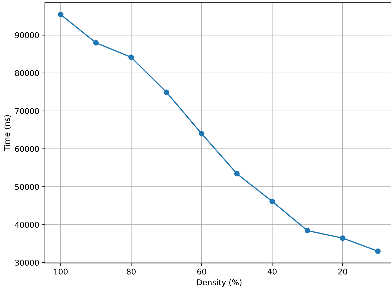
Matrix Density vs Time (lowThrust_12 - consec)
