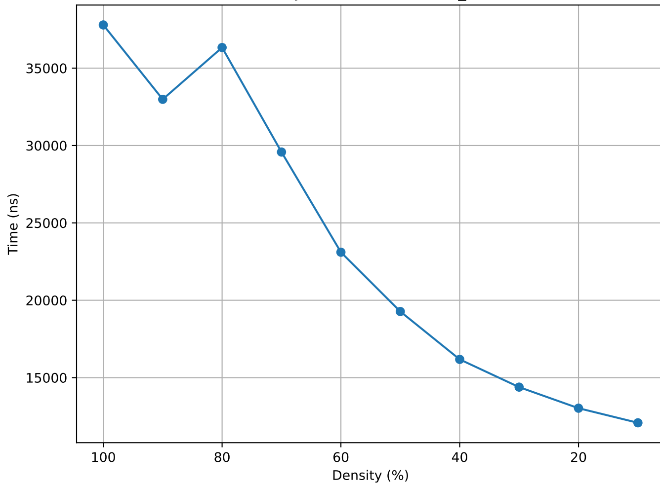
Matrix Density vs Time (lowThrust_3 - consec)
