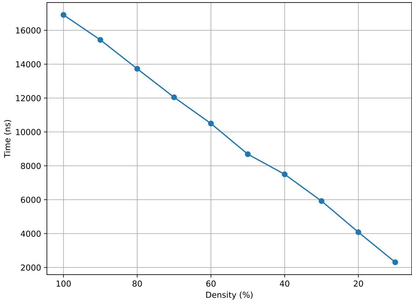
Matrix Density vs Time (lp_wood1p - random)
