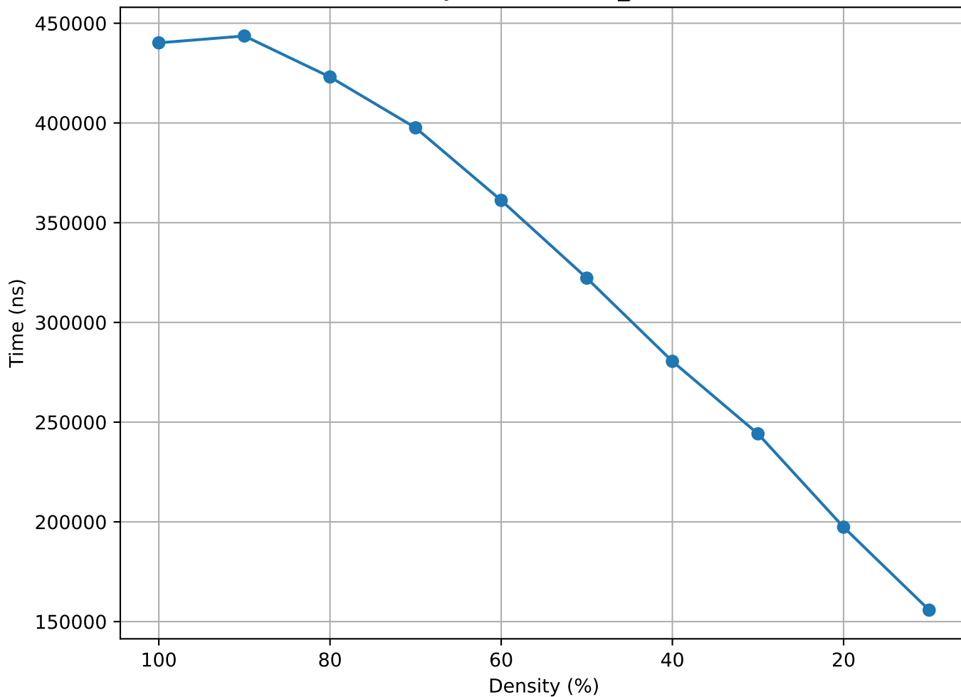
Matrix Density vs Time (std1_Jac2 - random)
