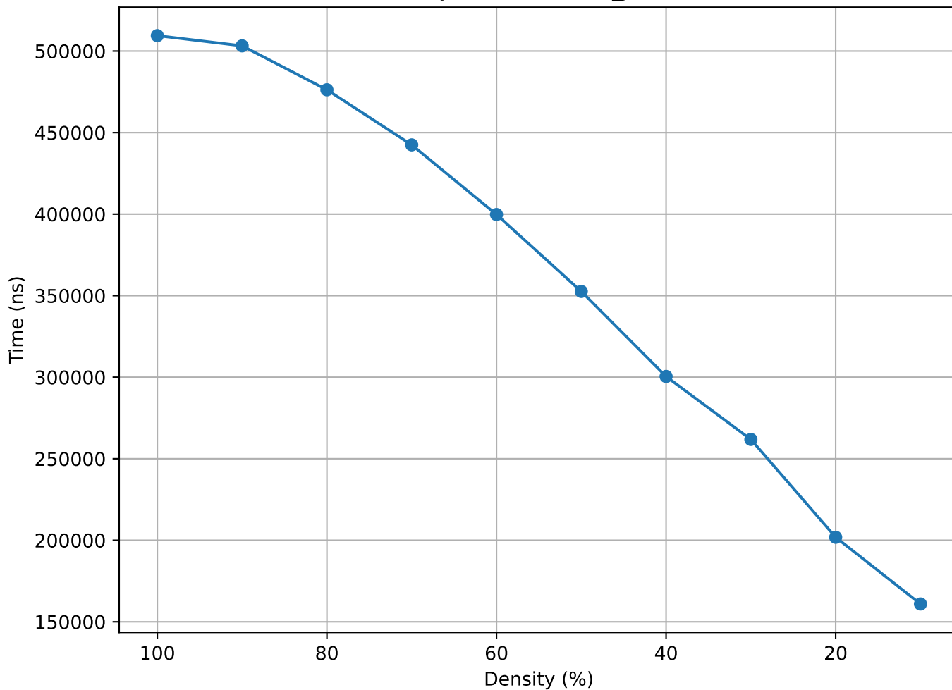
Matrix Density vs Time (std1_Jac3 - random)
