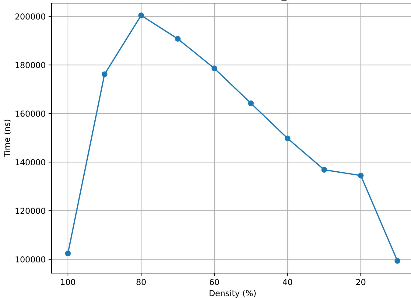
Matrix Density vs Time (lowThrust_10 - random)
