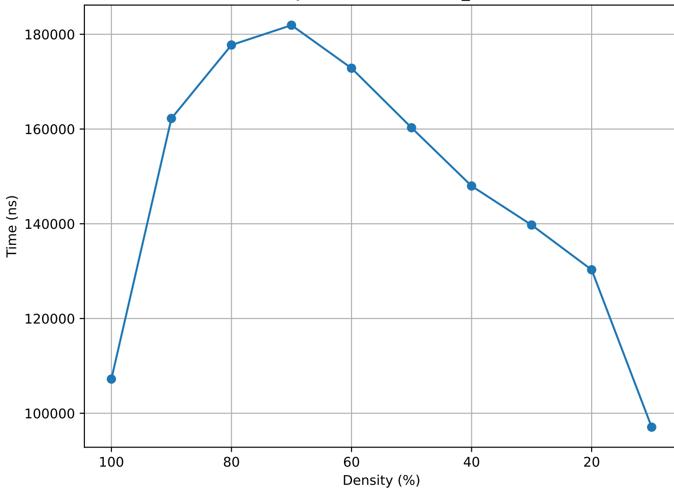
Matrix Density vs Time (lowThrust_12 - random)
